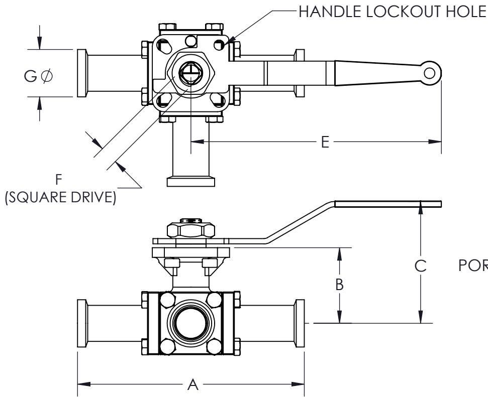
STC SERIES 3-WAY T-PORT DIMENSIONAL DATA
