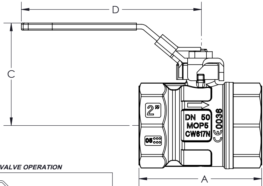
VALVE DIMENSIONS: SEL SERIES
